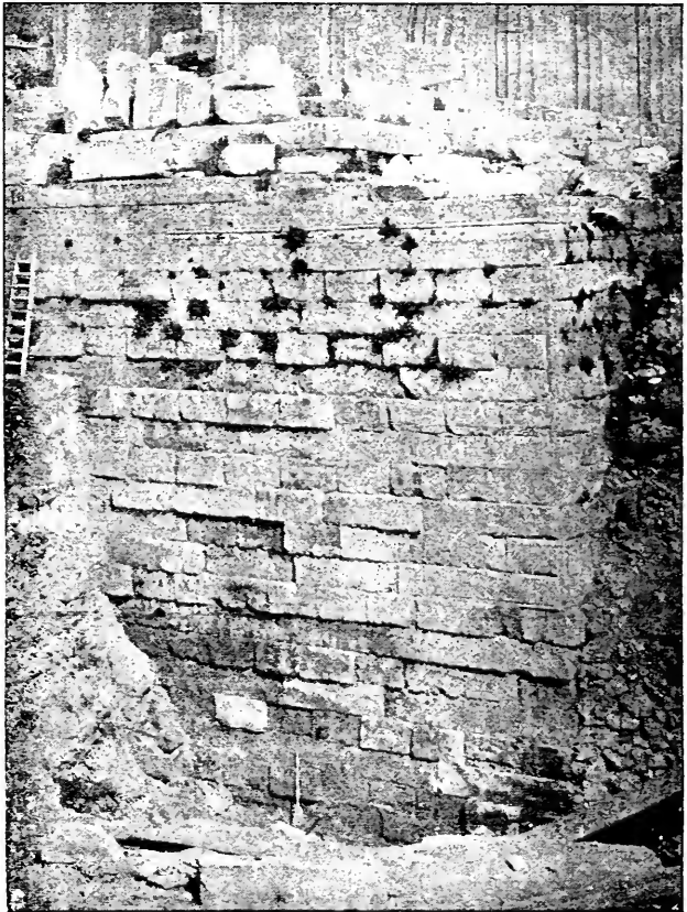
FIG. 63.—SOUTH-WEST CORNER OF FOUNDATIONS OF CIMON'S PARTHENON, AS SHOWN BY THE EXCAVATIONS (APRIL 1833).
